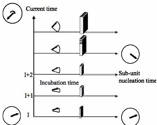
Figure 4: Illustrating the intermittent growth of a sheaf. If the waiting time since its last growth step is greater than the incubation time, then growth is resumed, and vice versa .
